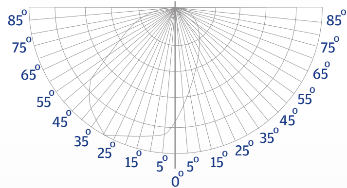
Angled Blades create an ultra-efficient Light Distribution Curve
